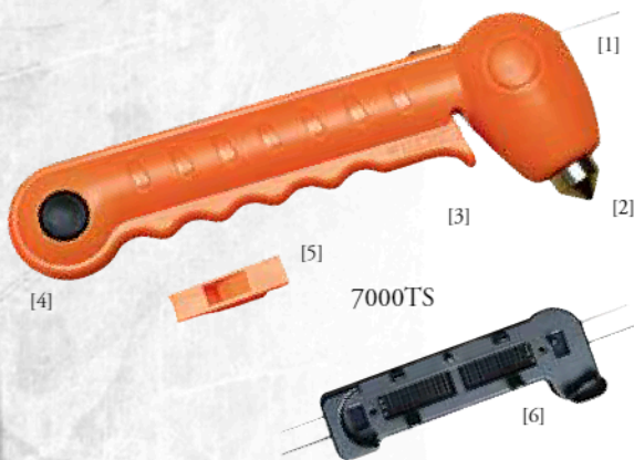
[1] Airbag deflator [2] Striking head [3] Seat belt cutter [4] Red LED light [5] Emergency whistle [6] Mounting kit
